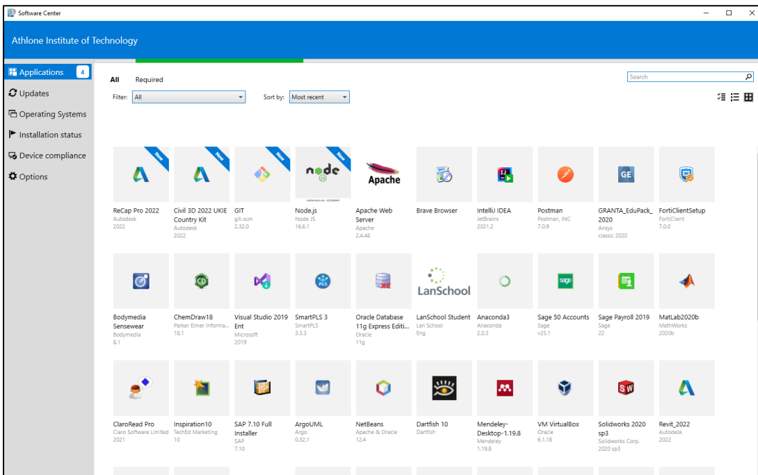
Figure 1: Software Centre
